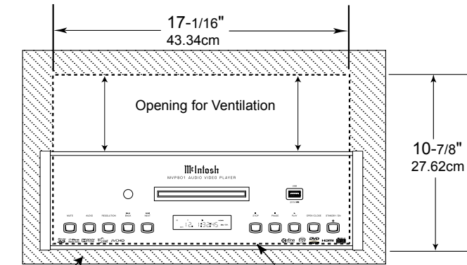
Cabinet Front Panel
