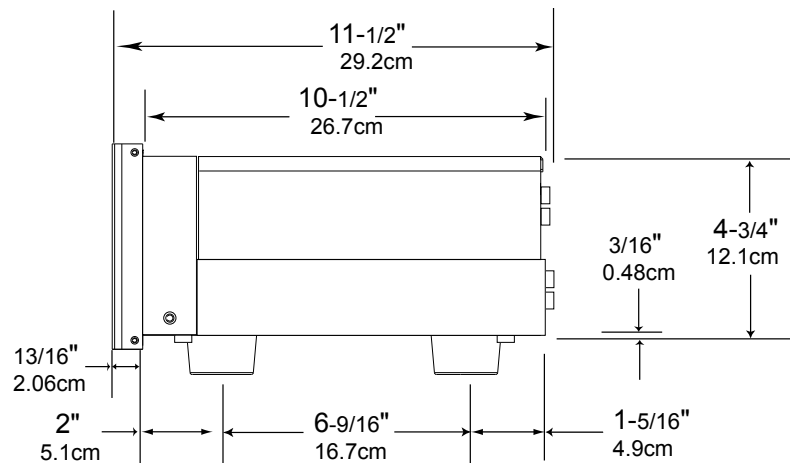
Side View of the MVP901
