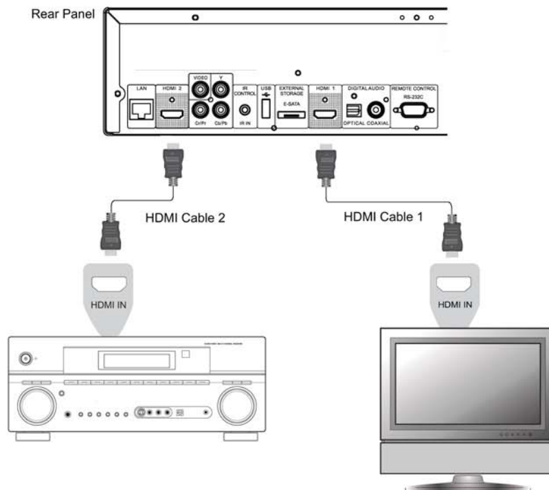
Method 10 – Dual HDMI Connection
