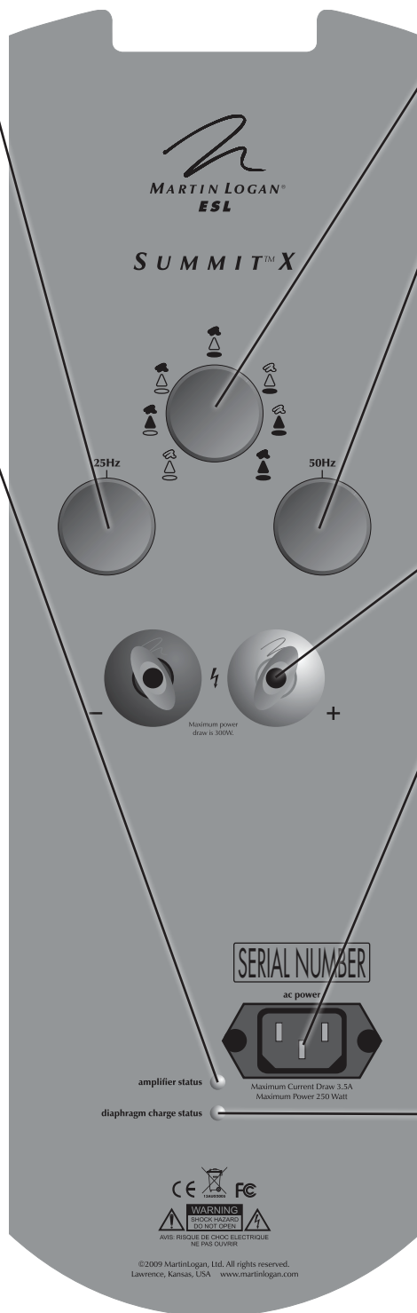
Figure 1. Summit X Controls and Connections
