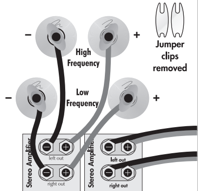
Fig. 4: Vertical bi-amplification connection. One channel shown.
