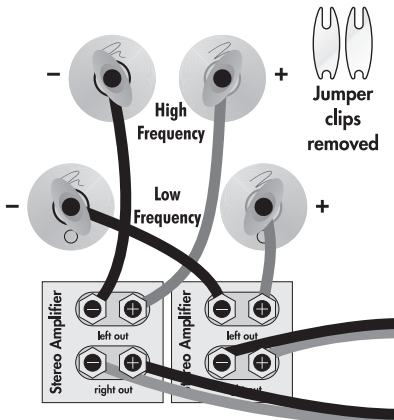
Fig. 3: Horizontal bi-amplification connection. One channel shown.
