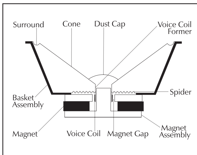
Figure 13. Cut away view of a typical moving coil driver. Notice the complexity due to the high number of parts.
