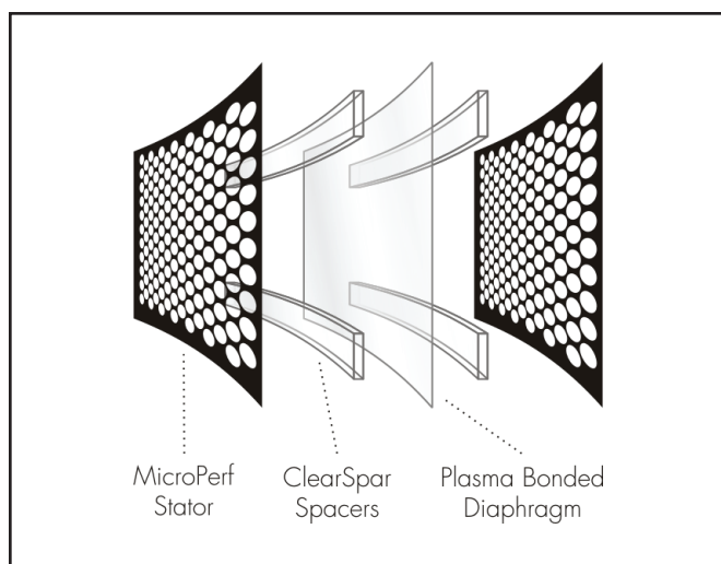
Figure 12. Cut away view of an XStat electrostatic transducer. Notice the simplicity due to minimal parts usage.
