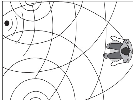
Figure 5-6. As can be seen here, point source concepts invite a great deal of room interaction. While delivering good frequency response to a large listening audience, imaging is consequently confused and blurred.
