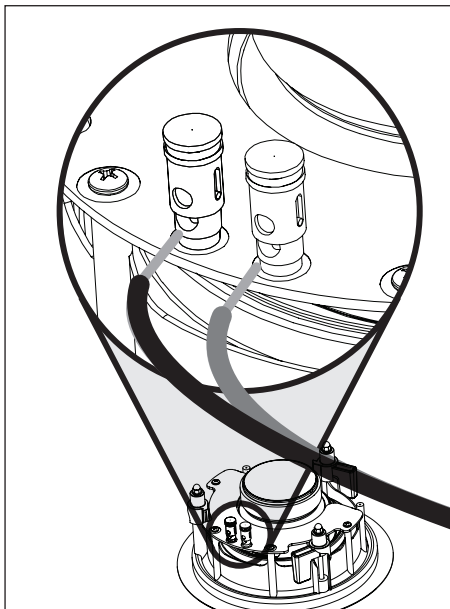
Figure 1. Raccordement du Helos 12.
