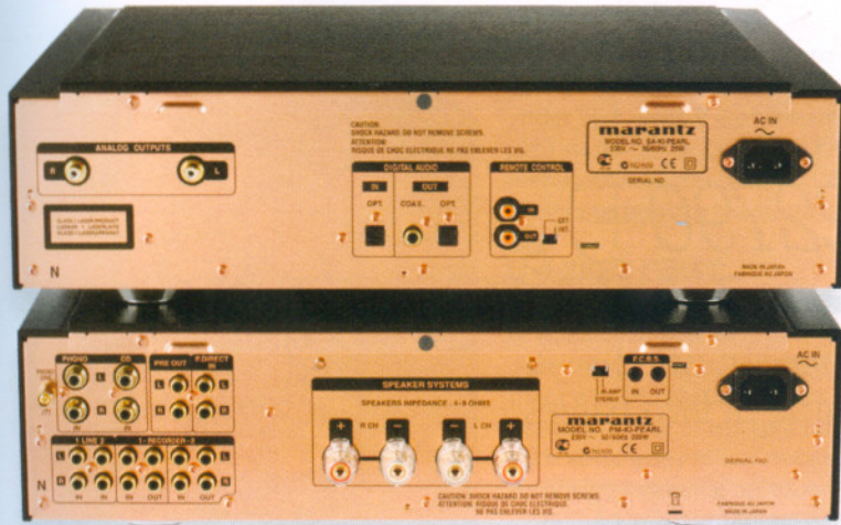
ABOVE: Single-ended analogue and digital outputs on the SCD player (top) join phono, three line and two tape inputs on the amp. Pre-out/power-in are included
