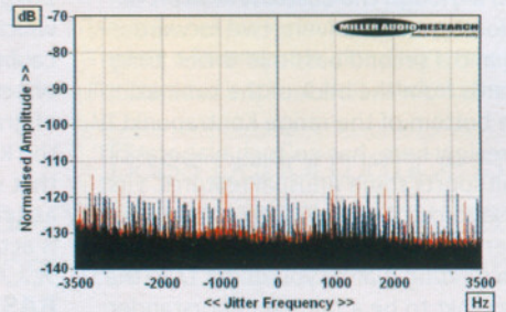
ABOVE: Jitter is a little lower at 220psec via SACD (red) than the 330psec via CD (black)
